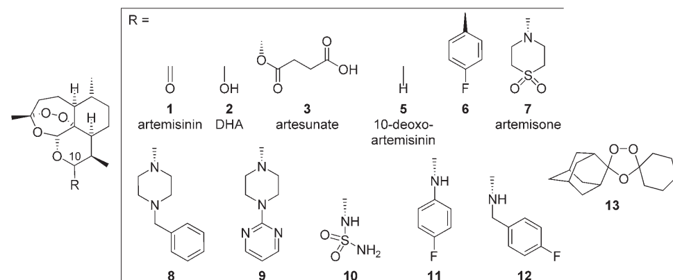
Figure 2. Artemisinins 1 – 12 and synthetic trioxolane 13 [51] used in this study.
